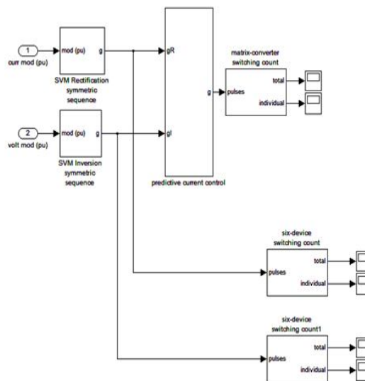
Fig 5: SVPWM Block
