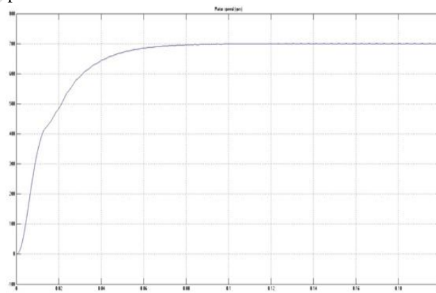
Fig 6: Speed Response
