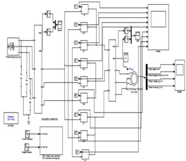
Fig 3. Simulation model of three phase matrix converter
