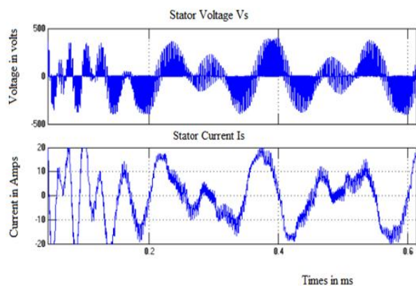
Fig 8: Stator voltage and current waveform
